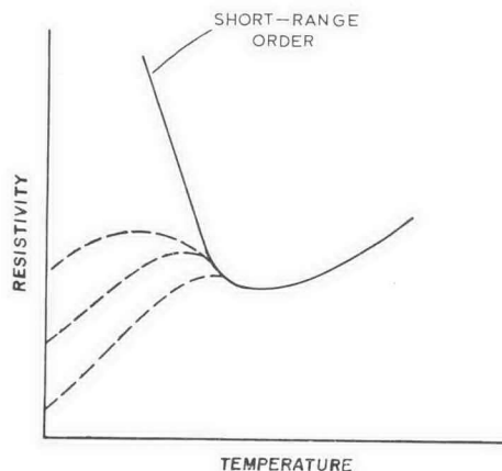
Resistivity-temperature curves for short-range order and K-state.
